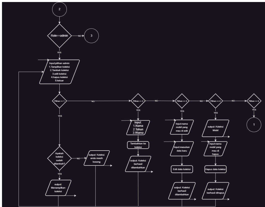
Flowchart menu admin
